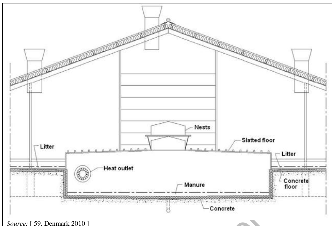
Figure 4.15: Scheme of the manure drying system in aviaries with a deep pit
