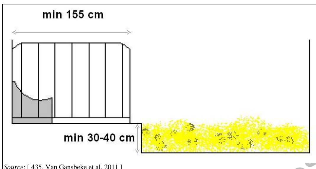
Figure 4.43: Scheme of the floor levels in bedded pens with feeding/lying boxes
