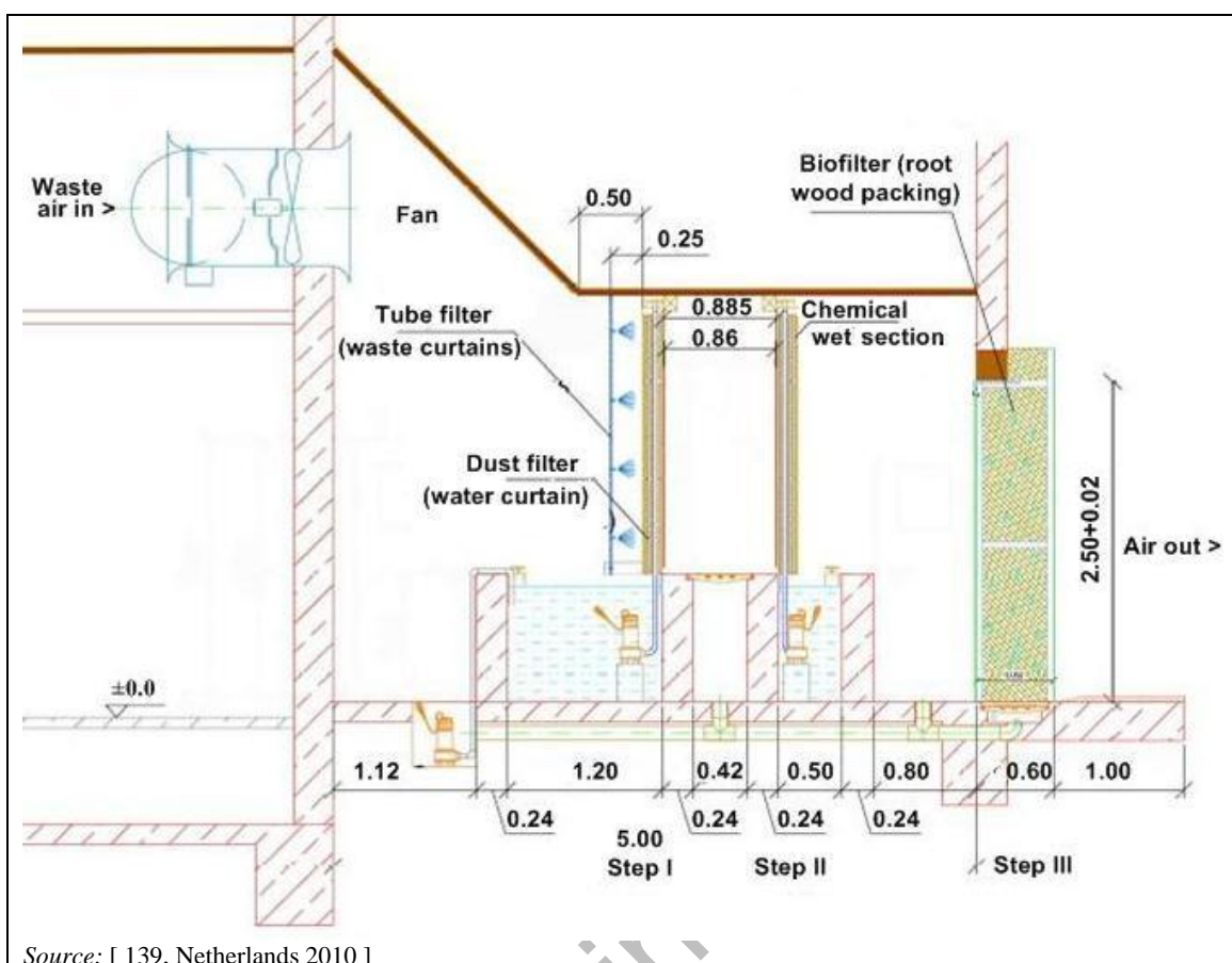
Figure 4.74: Combined multi-stage scrubber: water scrubber, wet acid scrubber and biofilter
