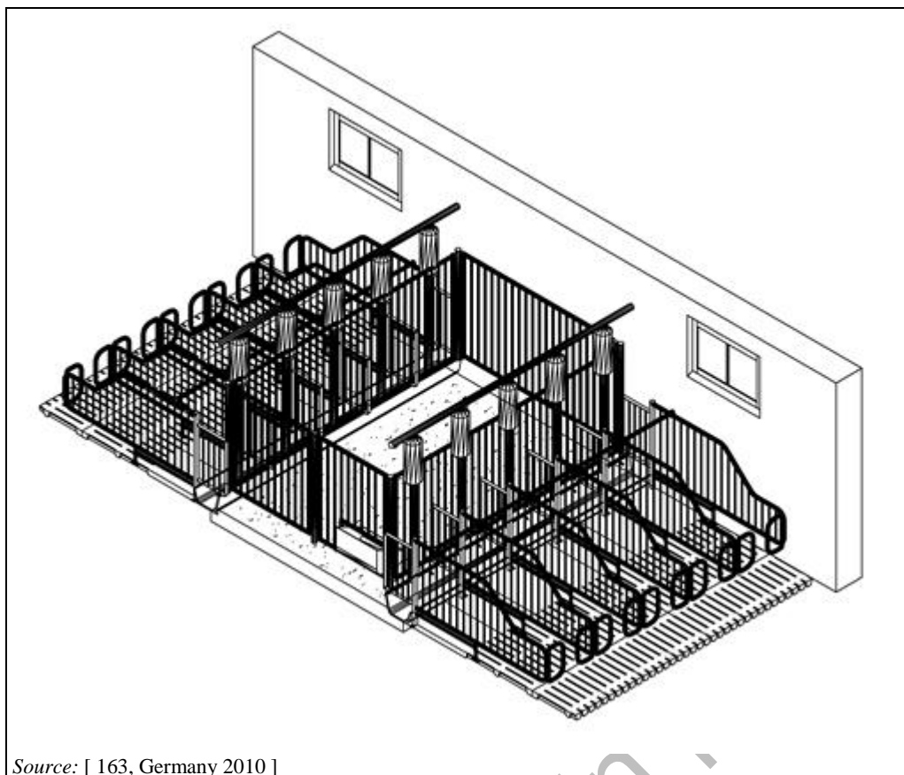
Figure 2.11: Individual housing of mating sows (service centre)
