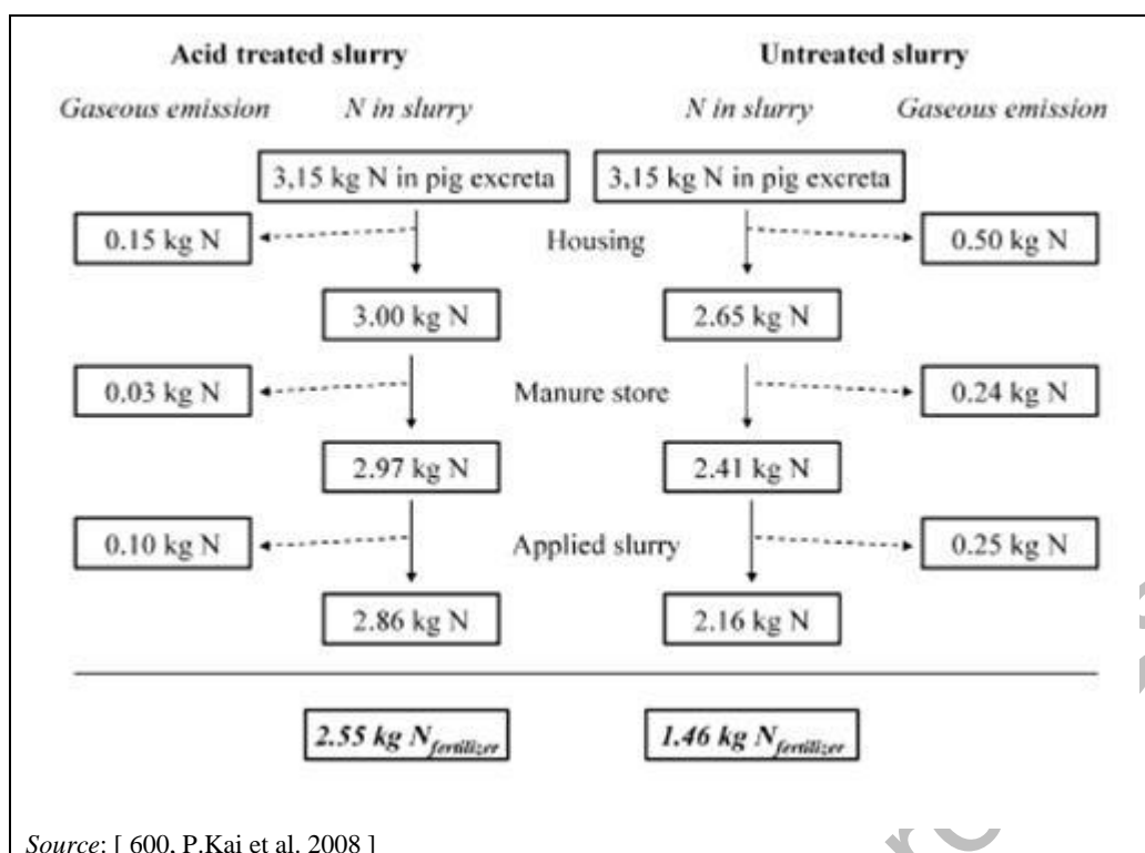
Figure 4.94: Whole-farm assessment of the slurry acidification effect on the available nitrogen for plant uptake
