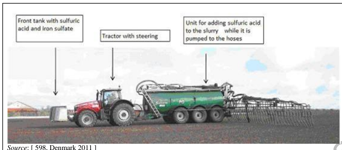
Figure 4.93: Equipment for slurry acidification during spreading
