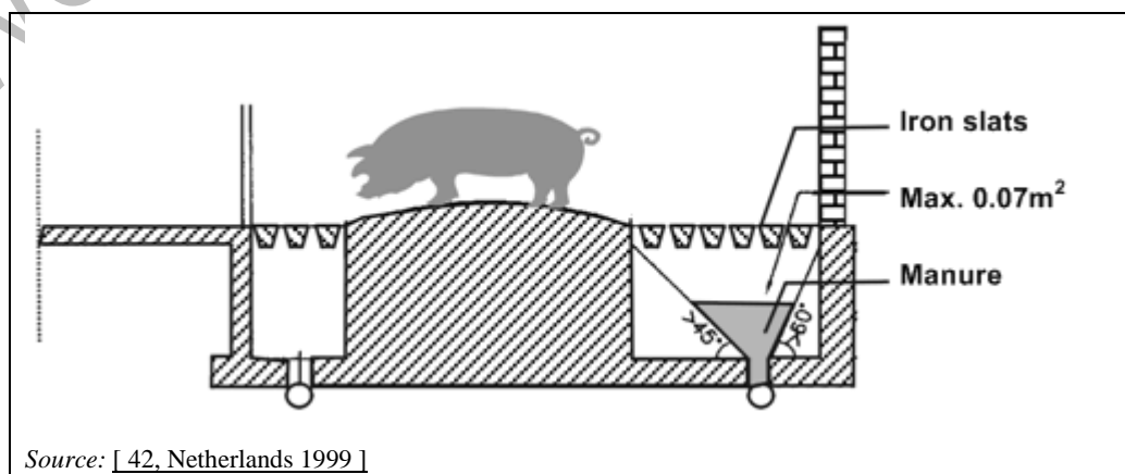
Figure 4.54: Convex floor with triangular metal slats in combination with discharge system and slanted walls in the manure channel
