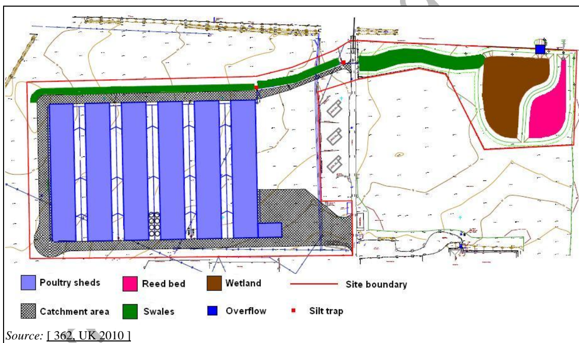
Figure 4.104: Location of a system of swales and wetland for a poultry farms
