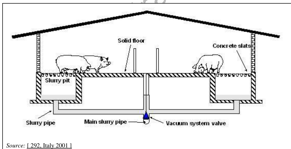
Figure 4.29: Partly slatted floor with a vacuum system
