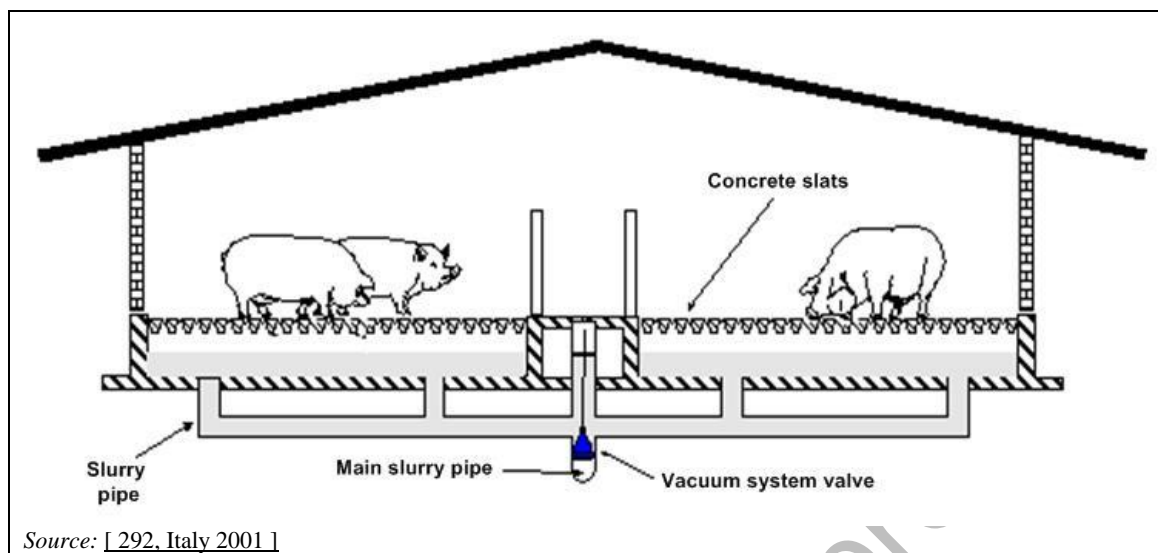
Figure 4.28: Fully slatted floor with vacuum system
