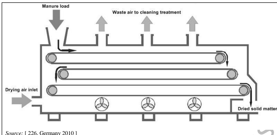
Figure 4.95: Scheme of a manure belt dryer
