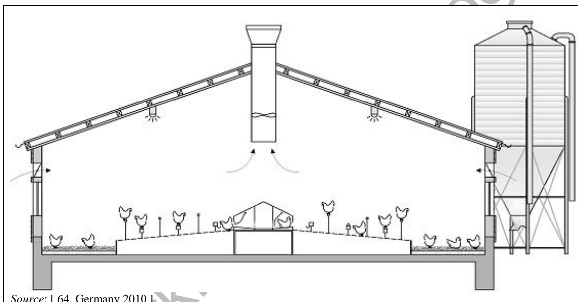
Figure 4.10: Schematic representation of a deep litter with manure pit housing system for laying hens
