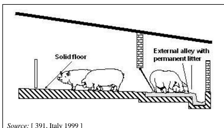
Figure 2.28: Solid concrete floor with external littered alley and manure channel
