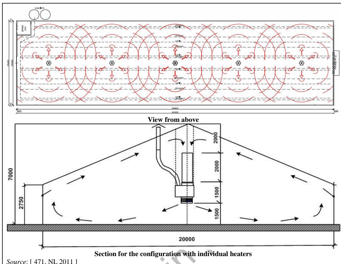
Figure 4.19: Plan and cross section of horizontal ventilation with recirculated air by indoor fans
