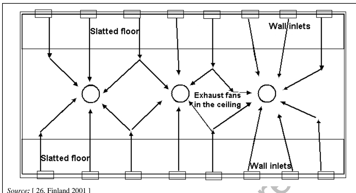
Figure 2.29: Schematic view of airflow in an exhaust ventilation system
