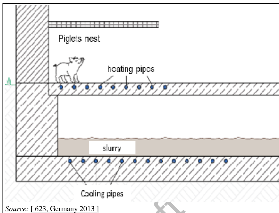
Figure 6.3: Scheme of slurry cooling in the shallow manure channels and heated piglet area
