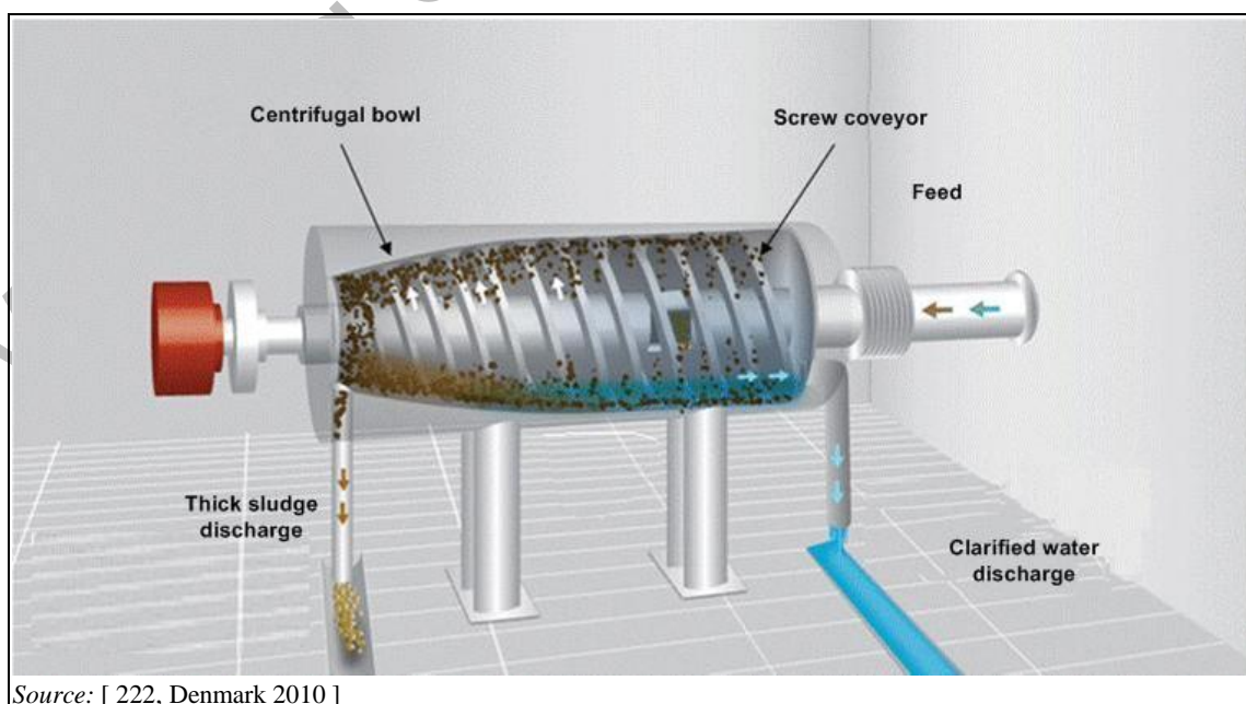
Figure 4.84: Schematic of a decanter-centrifuge for slurry separation
