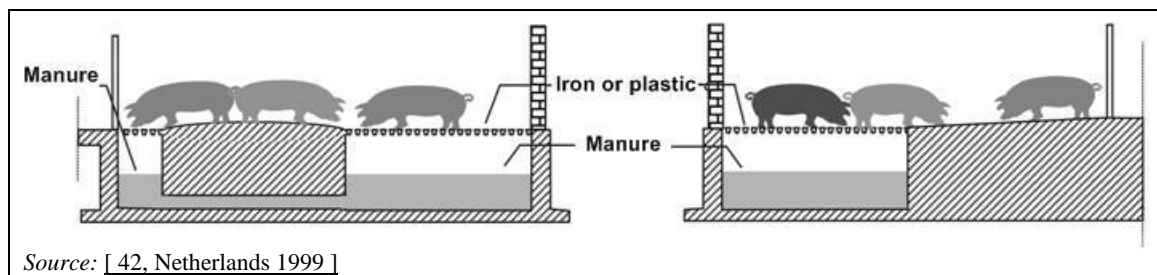
Figure 4.55: Partly slatted floor with convex or sloped concrete floor
