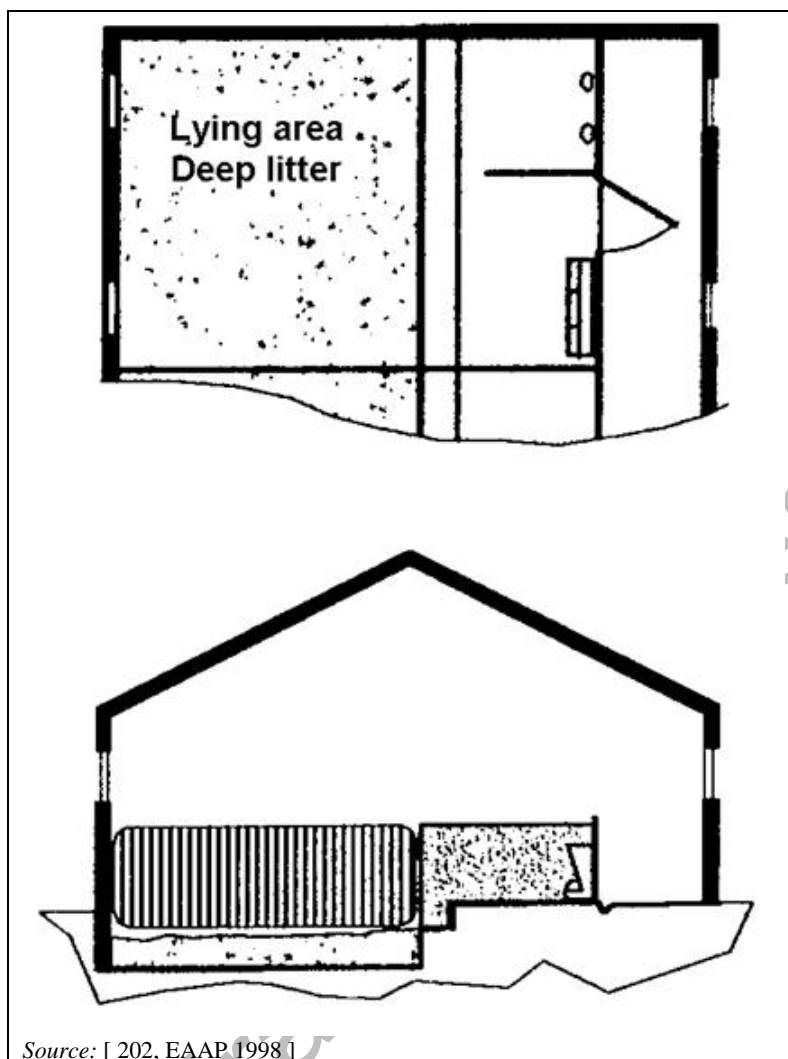
Figure 2.27: An example of a solid concrete floor system for fattening pigs
