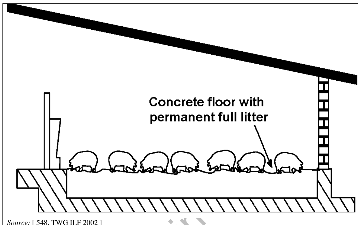
Figure 4.65: Pens with solid concrete straw-bedded floor and natural ventilation
