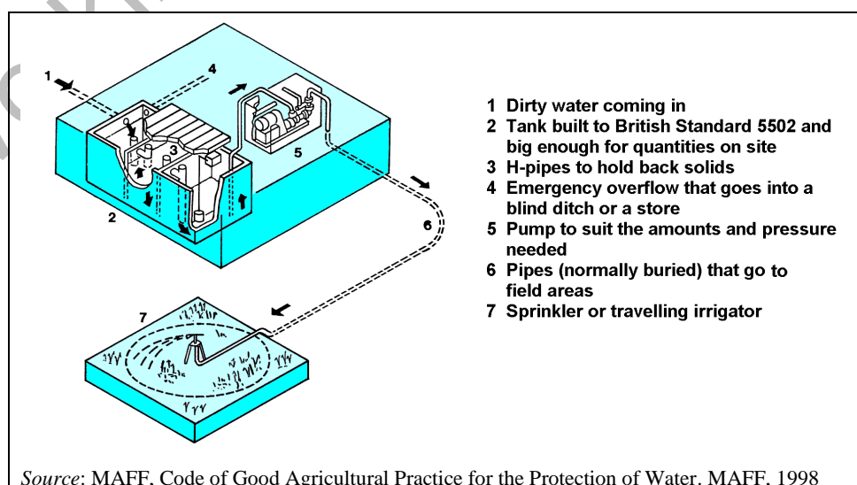
Figure 4.105: Example of sprinkler or travelling irrigation system
