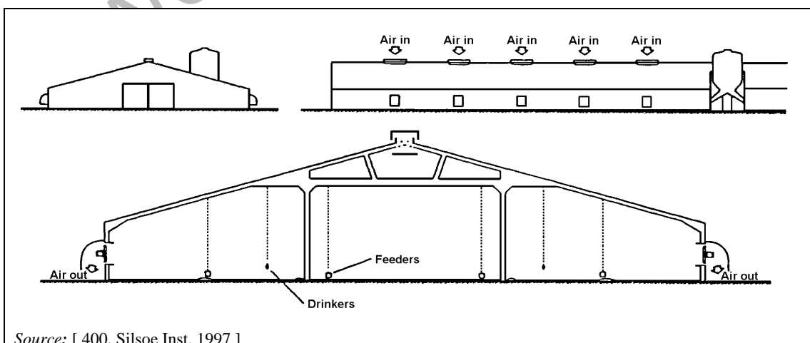
Figure 2.8: Example of schematic cross section of a common broiler house
