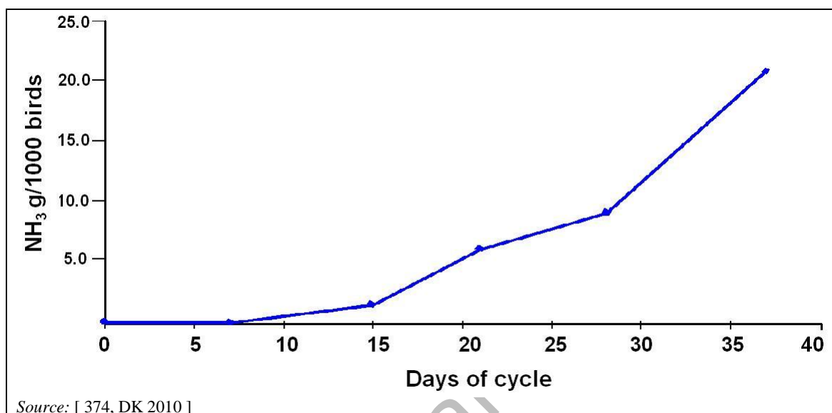
Figure 4.72: Ammonia emissions from a broiler house
