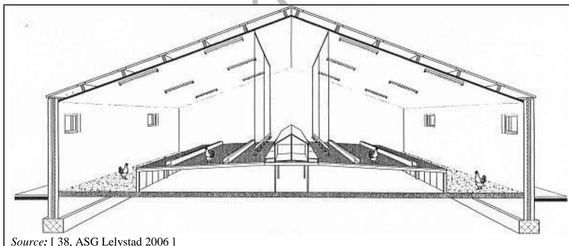
Figure 2.6: Schematic cross section of a single-tiered non-cage system
