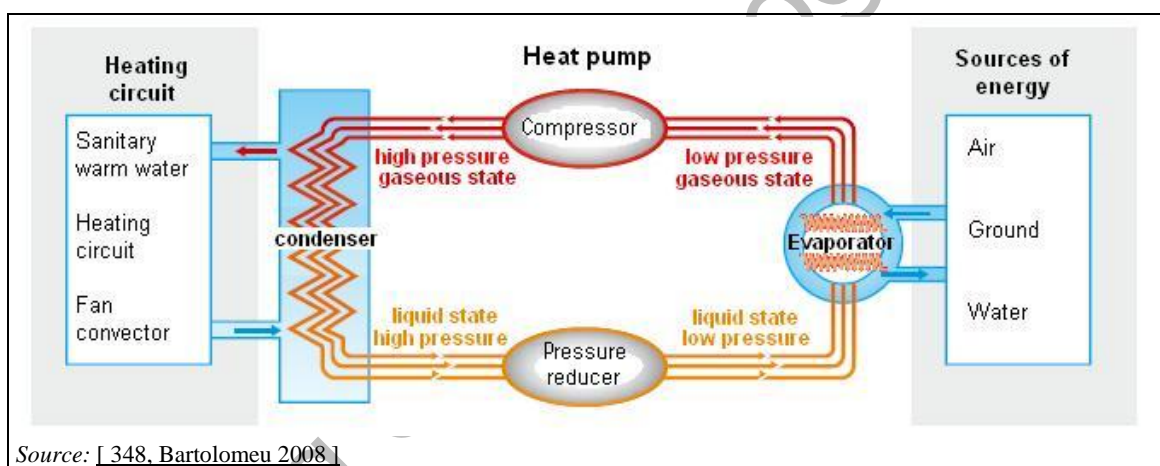
Figure 2.51: Operating principle of a heat pump
