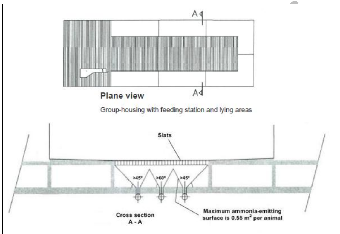
Figure 4.35: Cross section and plane view of the floor in a housing system for gestating sows with a manure channel with slanted walls
