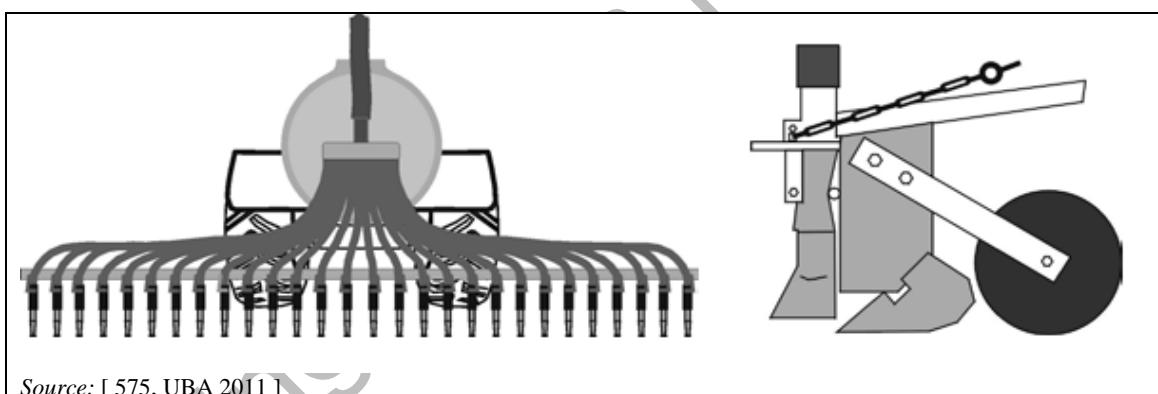
Figure 4.100: Scheme of an open slot injector
