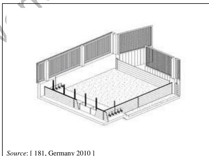
Figure 4.58: Housing system with deep litter for weaned piglets
