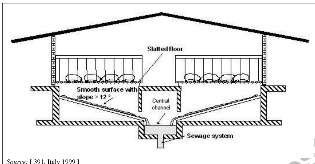
Figure 4.56: Flat decks or pens with concrete sloping underground to separate faeces from urine
