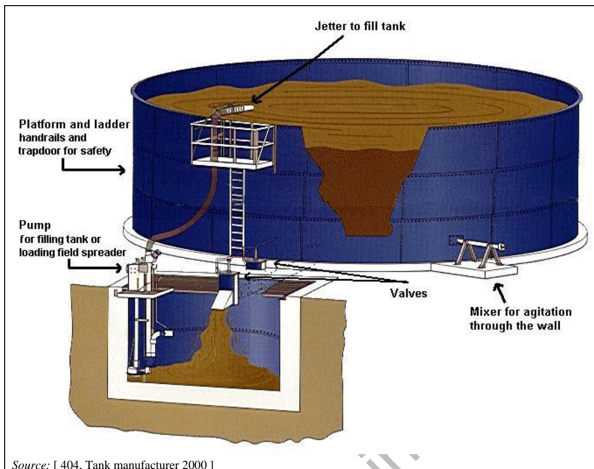
Figure 2.35: Example of above-ground slurry tank with an underground receiving pit
