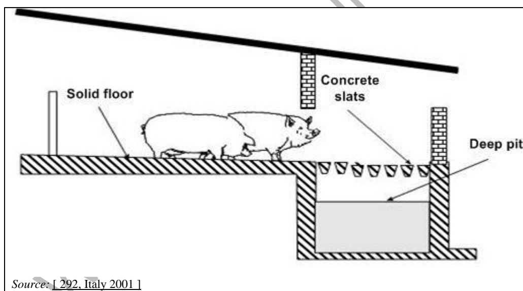
Figure 4.38: Solid concrete floor and fully slatted external alley with storage pit underneath
