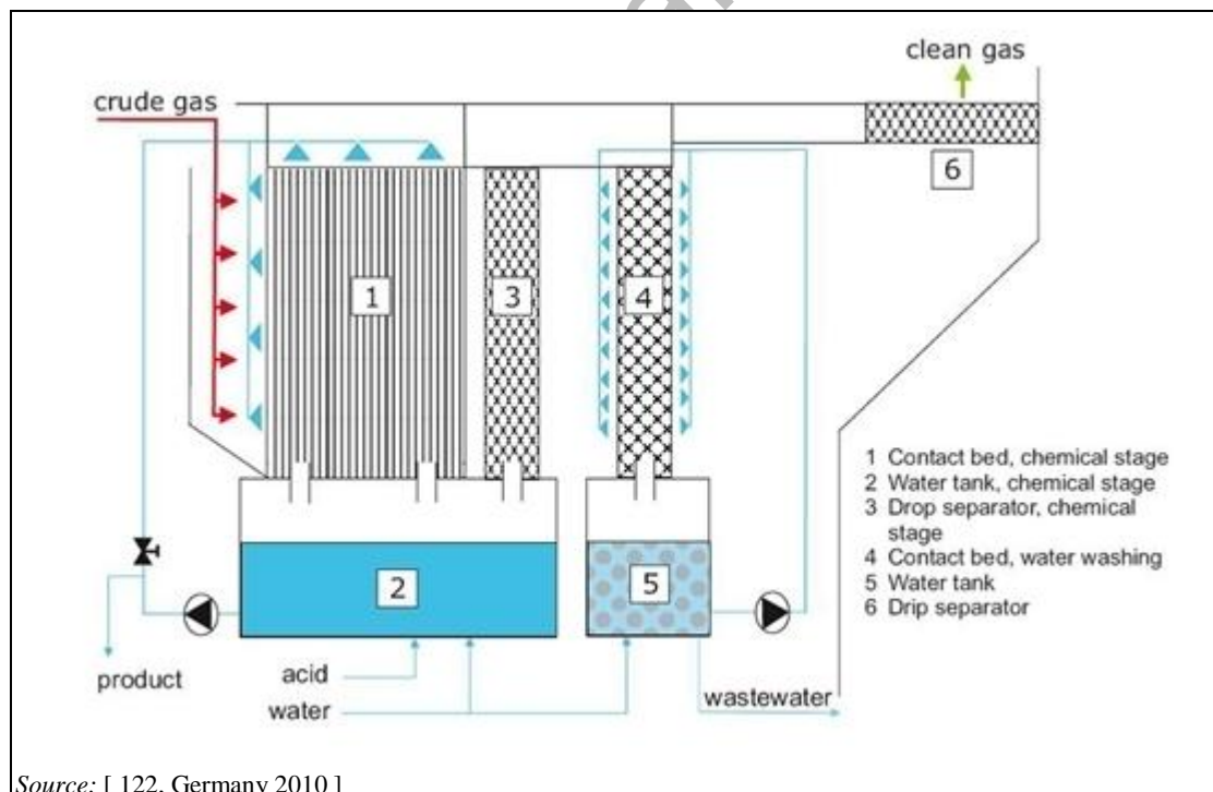
Figure 4.73: Two-stage air scrubber with combined acid scrubber and bioscrubber
