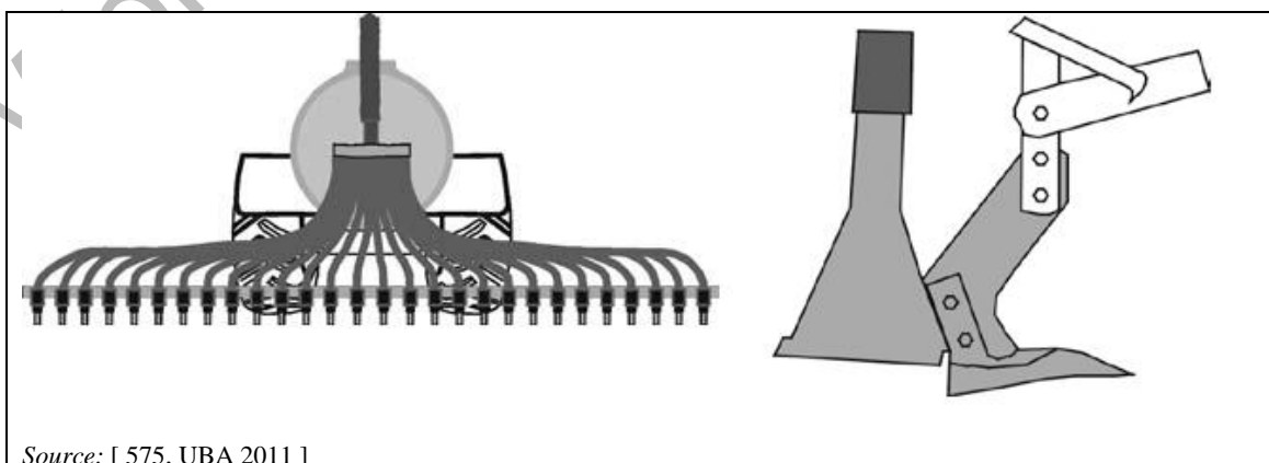
Figure 4.99: Scheme of a trailing shoe spreader
