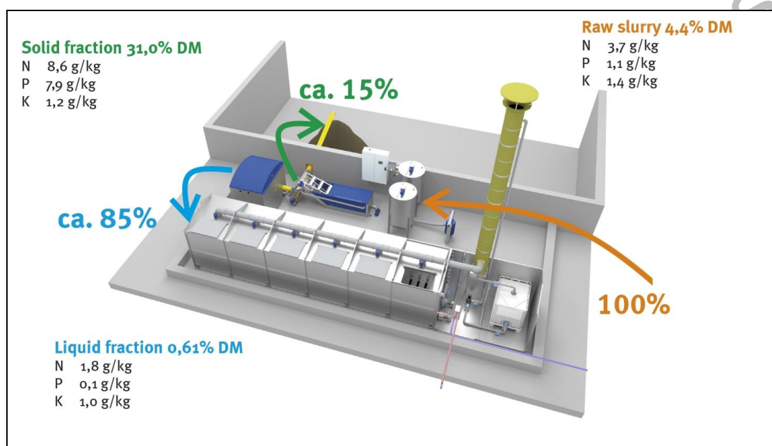
Figure 4.88: Mass balance and composition of the different streams resulting from a combination of a mechanical separation stage with flocculation and a biological aeration treatment with serial tank configuration
