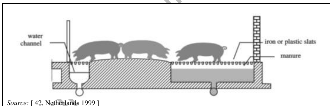
Figure 4.53: Partly slatted floor with shallow manure pit and a water channel for spoiled drinking water in combination with a convex floor
