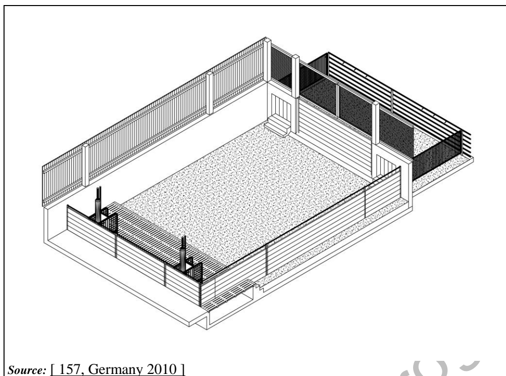
Figure 4.41: Littered floor with slatted feeding area
