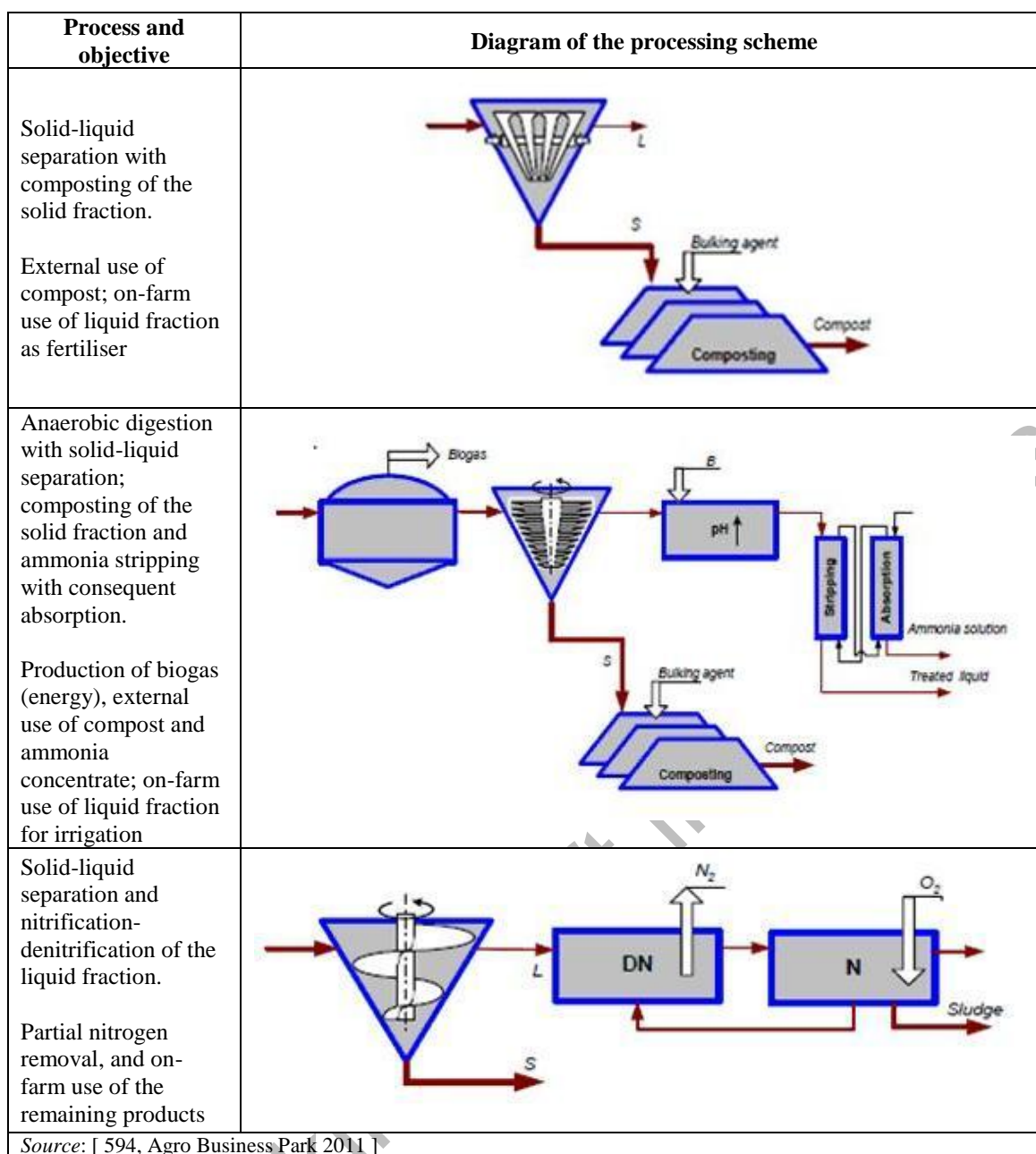
Figure 4.82: Examples of manure processing strategies
