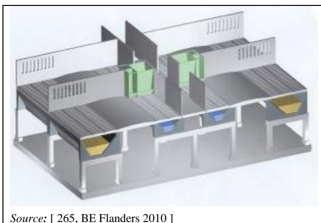
Figure 2.24: Pen design for fattening pigs with partly slatted (convex) floor and solid area in the centre
