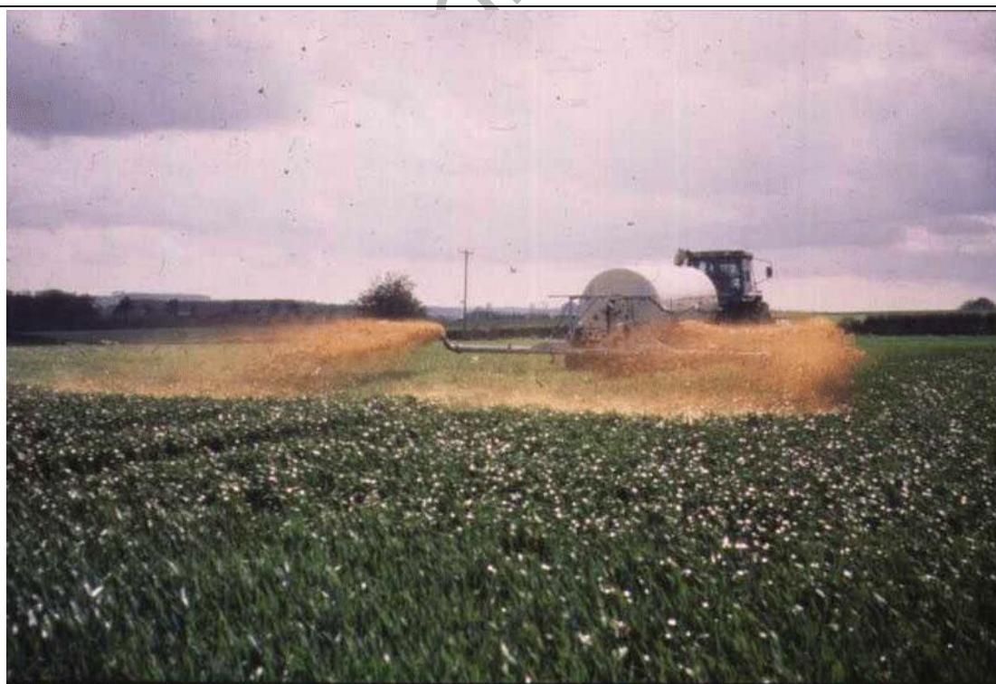
Figure 2.41: Example of a broadcast technique with low trajectory and low pressure
