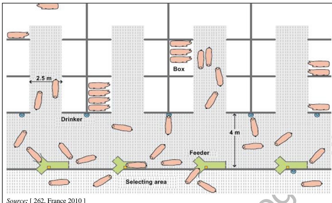
Figure 2.16: Layout of a pen for gestating sows fed with an electronic feeder
