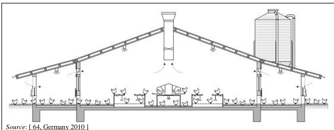
Figure 4.11: Schematic representation of a deep litter with manure pit housing system for laying hens, with veranda and forecourt free range
