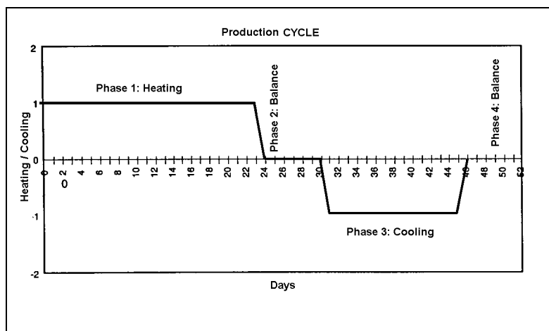
Figure 4.8: Graphic representation of the working principle of the 'combedeck system' during one broiler production cycle
