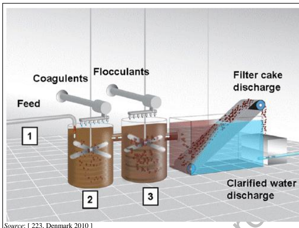
Figure 4.85: Schematic representation of a coagulation-flocculation pretreatment for slurry separation
