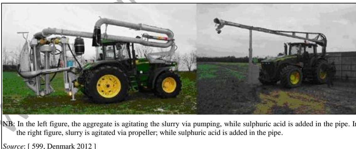
Figure 4.92: Systems for slurry acidification directly in the storage tank
