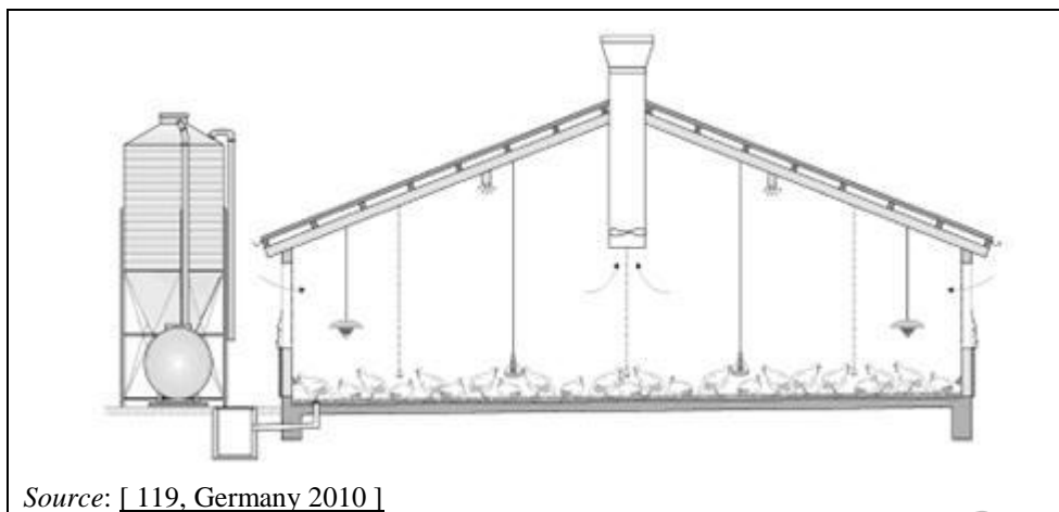
Figure 4.26: Scheme of a natural ventilated house for turkeys fattening
