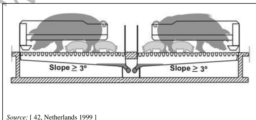
Figure 4.49: Fully slatted floor with manure pan
