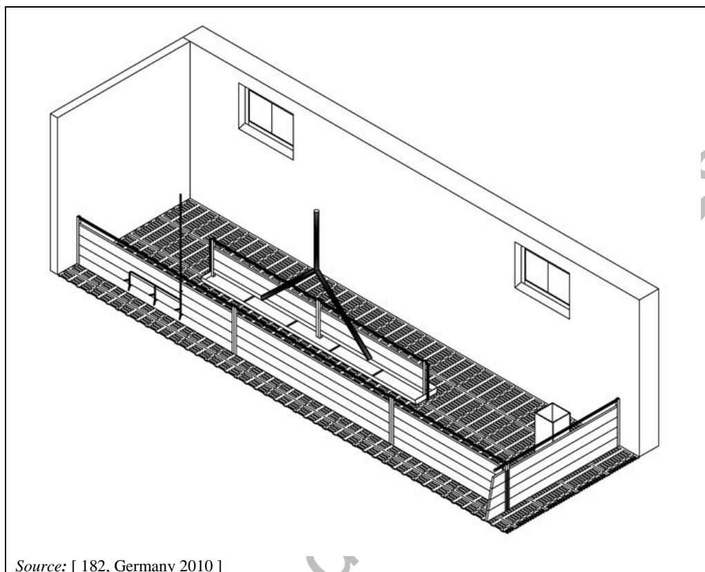
Figure 2.20: Schematic picture of a fully slatted floor pen for weaners
