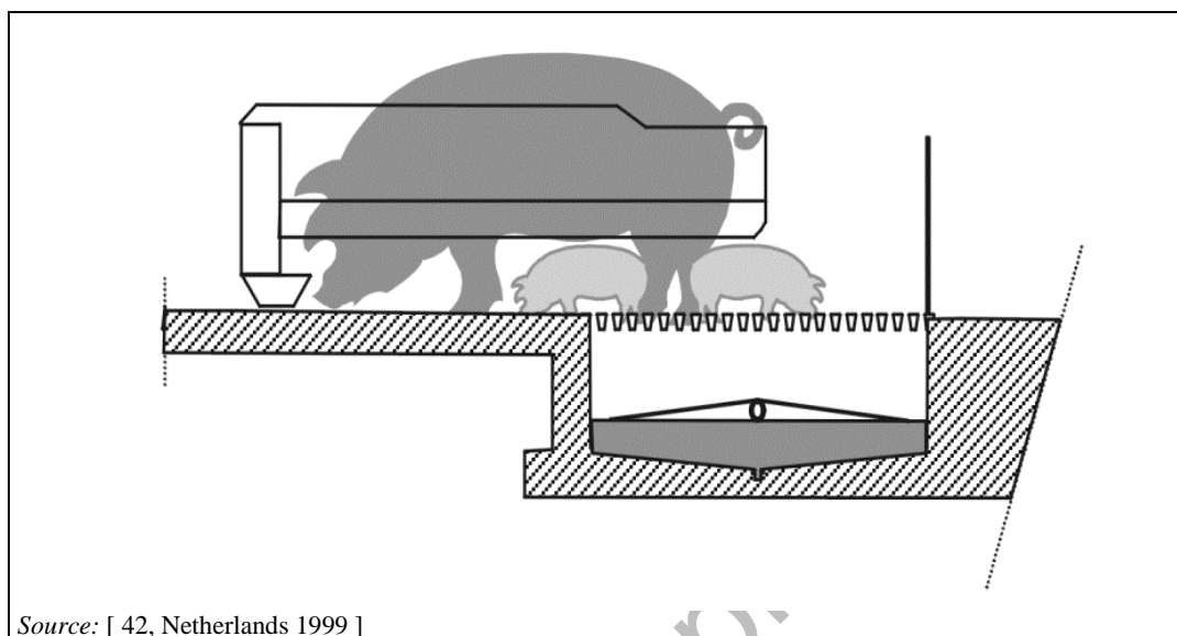
Figure 4.45: Farrowing crate with partly slatted floor with a manure scraper
