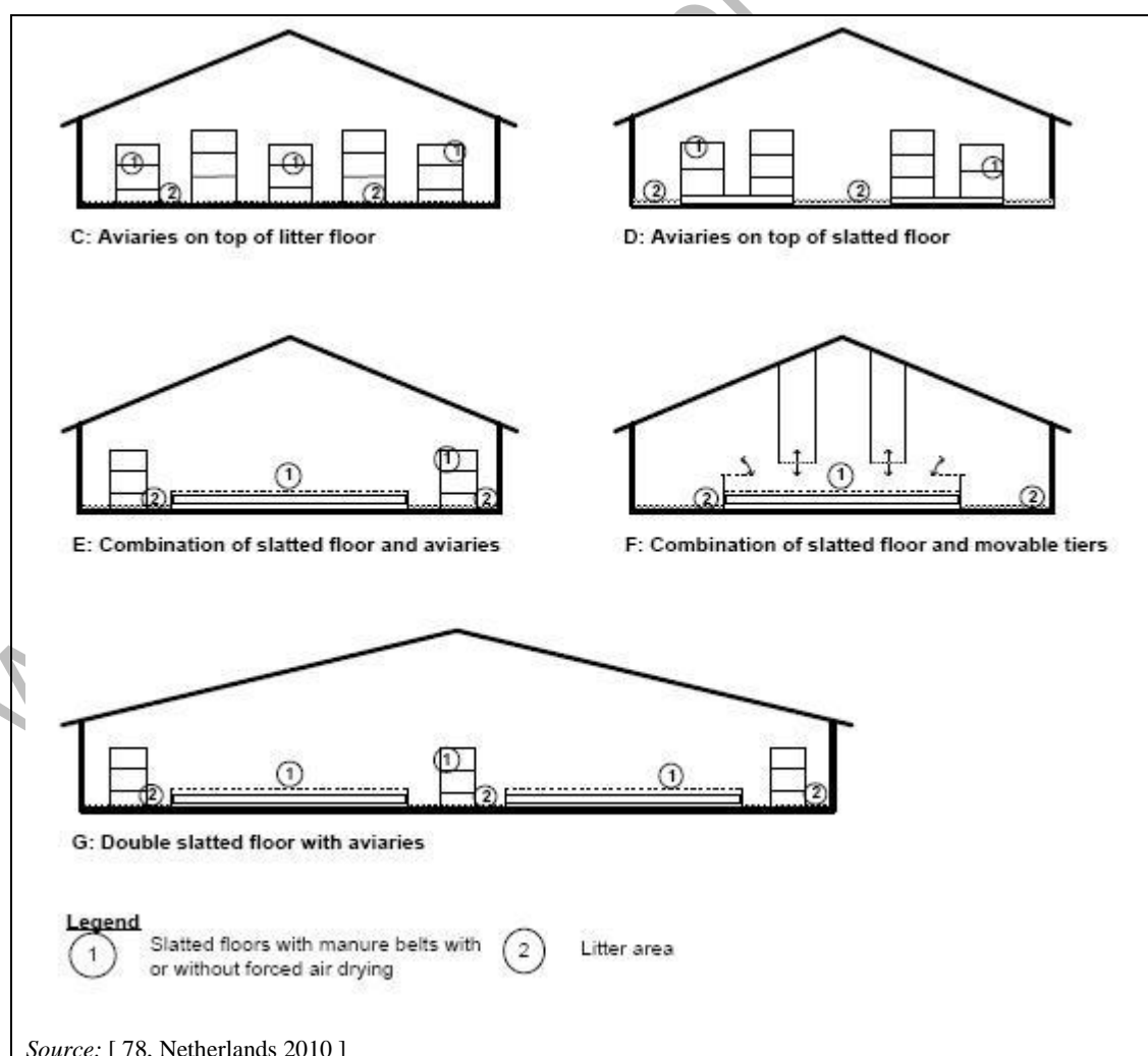
Figure 4.16: Combinations of slatted floors in aviaries
