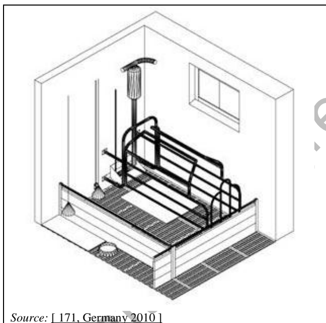
Figure 4.44: Farrowing crate with partly slatted floor (solid floor in the lying areas)
