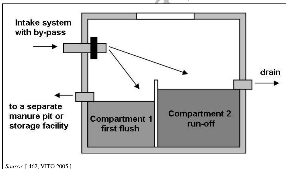
Figure 4.103: Scheme of a first flush system
