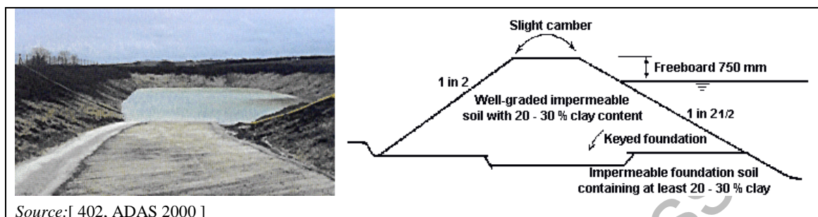
Figure 2.36: Example of earth-banked slurry store, and design features
