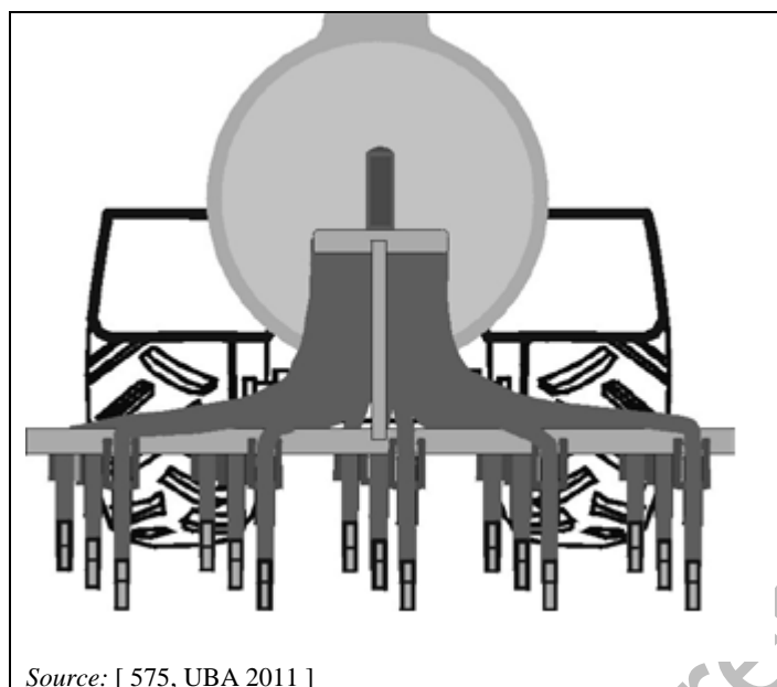
Figure 4.101: Scheme of an closed slot injector
