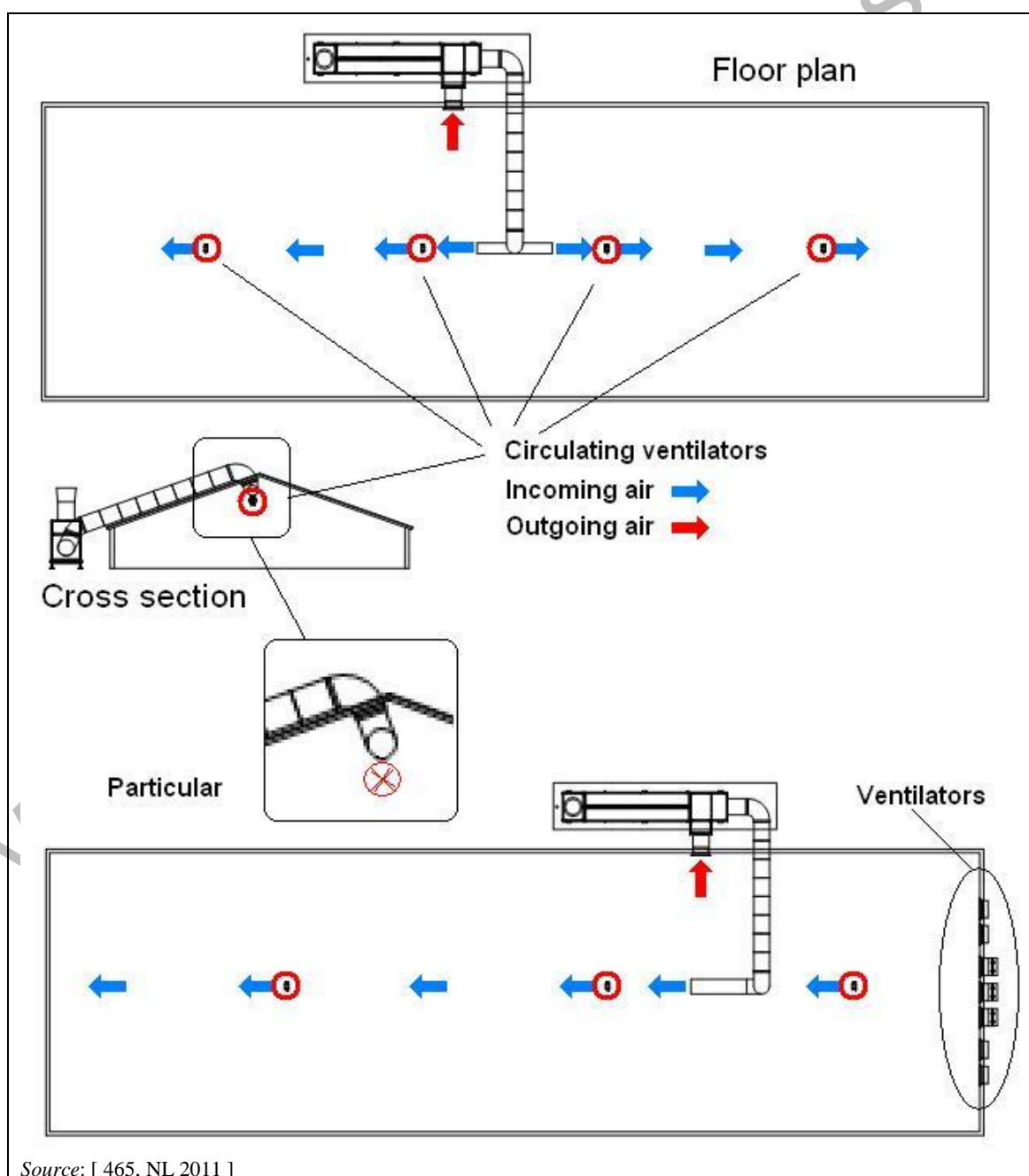
Figure 4.18: Examples of layouts for systems of circulating fans and heat exchanger
