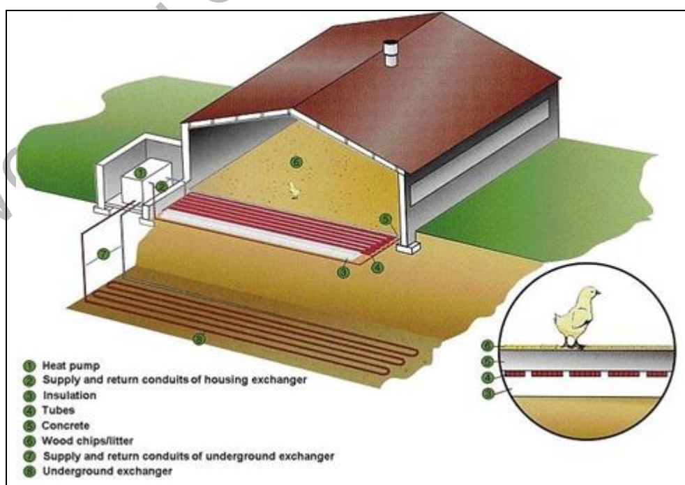
Figure 4.7: Schematic representation of a heat recovery system installed in a broiler house
