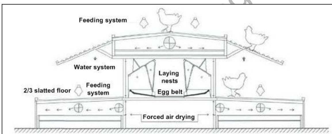
Figure 4.25: Scheme of an additional tier over the nests in an aviary system
