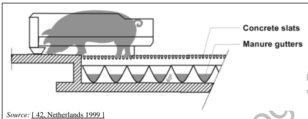
Figure 4.36: Partly -slatted floor with flushing gutters in individual mating/gestating sow housing
