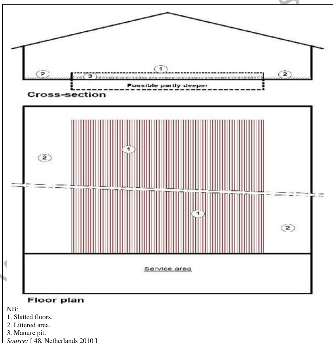
Figure 4.17: Cross section of the housing system with a deep litter and a manure pit
