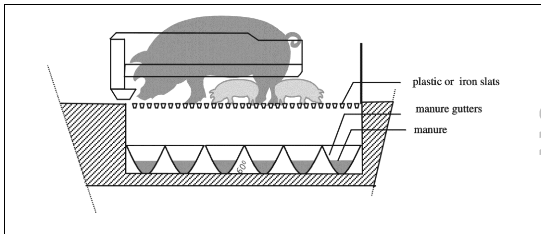
Figure 4.46: Flushing system with manure gutter
