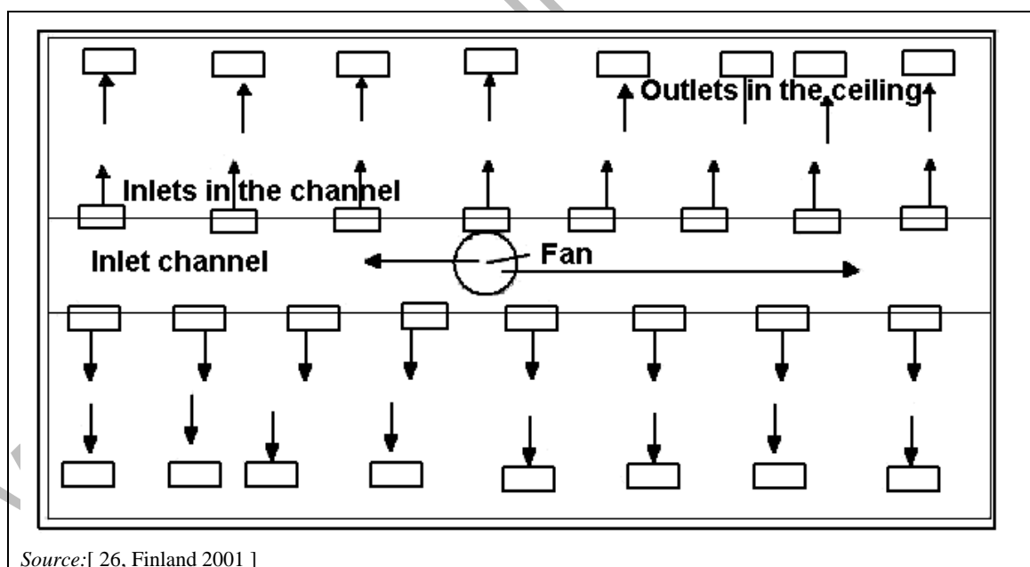
Figure 2.30: Schematic view of airflow in a pressure ventilation system
