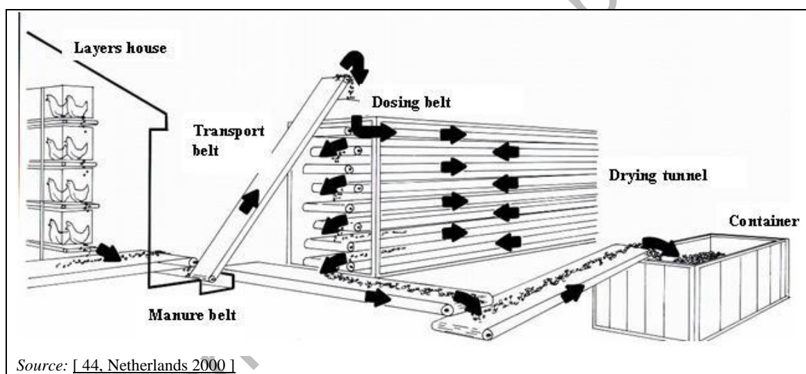
Figure 4.90: Principle of external drying tunnel with perforated manure belts
