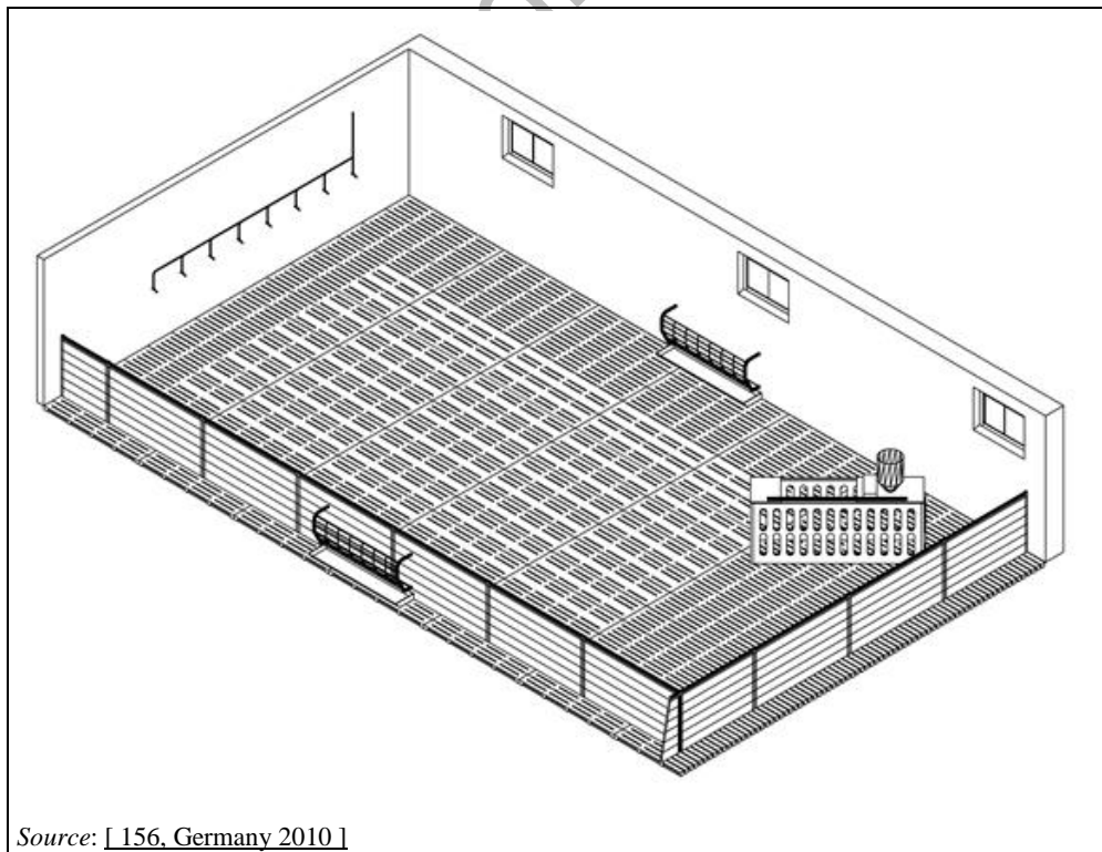
Figure 2.15: Example of group housing for mating and gestating sows with perforated lying area (perforation in the lying area <15 %)
