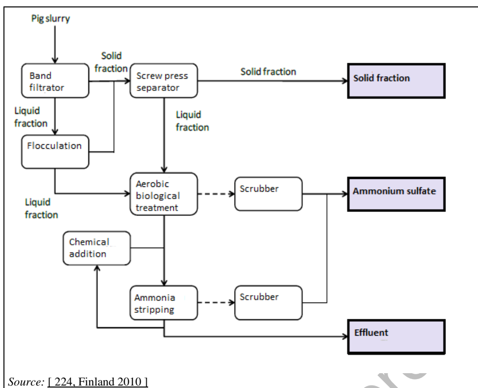
Figure 6.6: Schematic representation of the combined treatment system including solid separation step, biological treatment procedure and ammonia stripping stages
