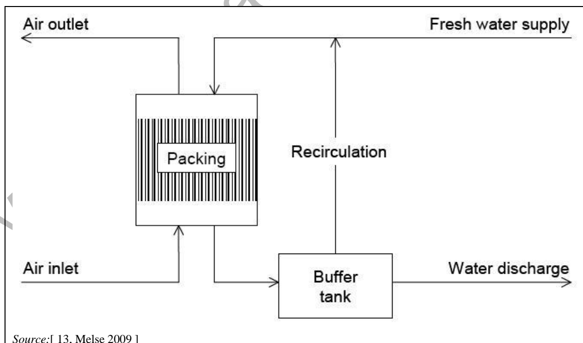
Figure 2.32: Schematic representation of a wet scrubber
