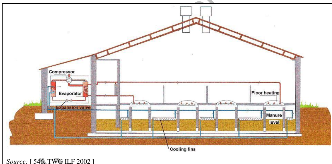
Figure 4.31: Manure surface cooling fins
