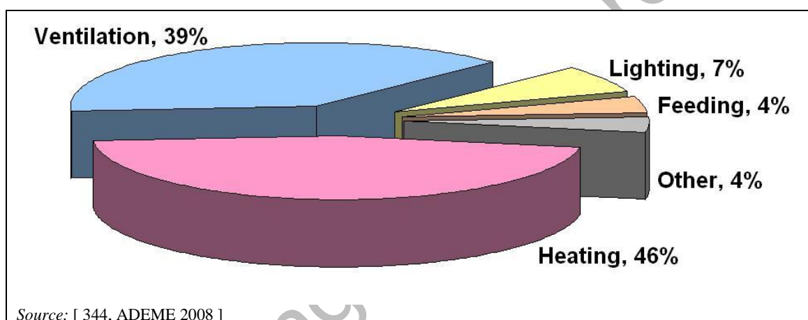
Figure 3.2: Breakdown of electricity consumption on pig farms in France
