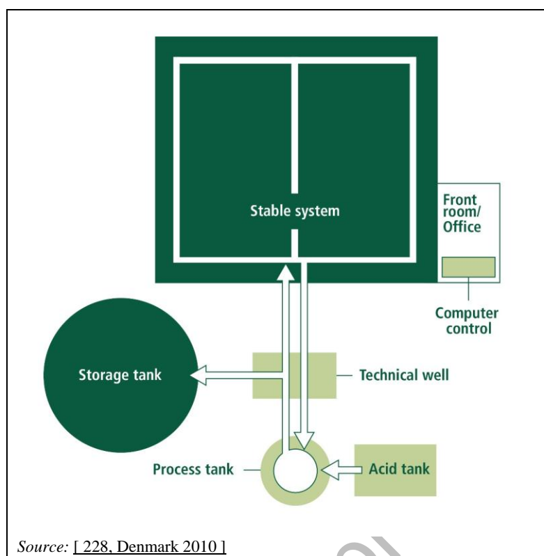
Figure 4.91: Schematic representation of a slurry acidification system
