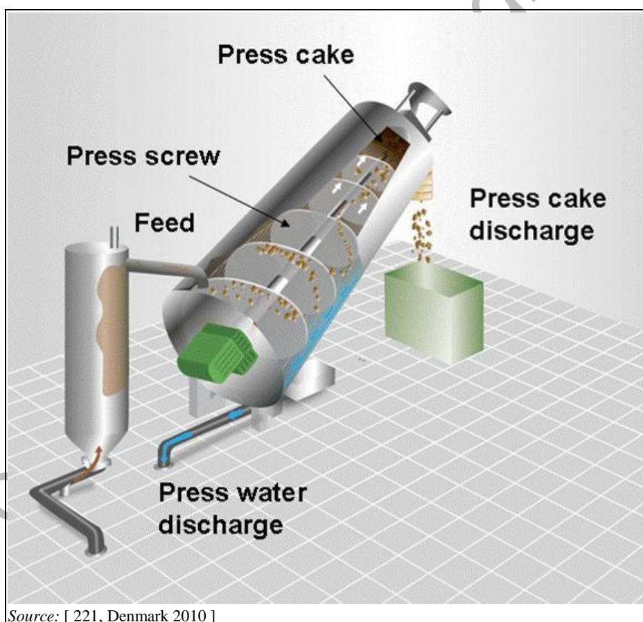
Figure 4.83: Screw press scheme
