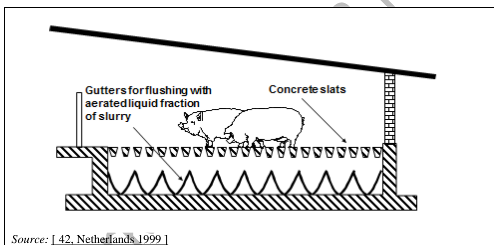
Figure 4.32: Fully slatted floor with flushing gutters
