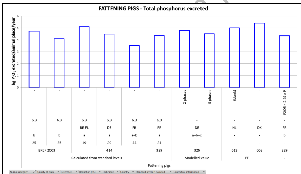
Figure 9.6: Total phosphorus excreted from fattening pigs
